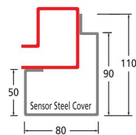
Surface Mounted SKB G Guide
