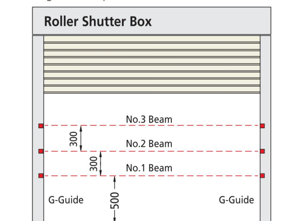
Single or Multiple Beams Installation
