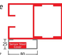
Wall To Wall Mounted SKB C-150 Guide
