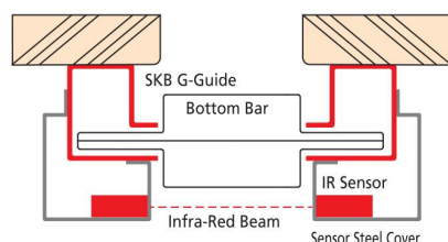
Drawing Shown Surface Mounted SKB G-Type Guide
